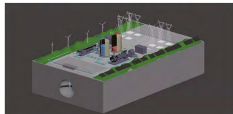
成功签约盐穴压缩空气储能电站(100MW)总承包项目 SIGNED AN EPC CONTRACT FOR 100MW SALT CAVERN COMPRESSED AIR ENERGY STORAGE (CAES) POWER PLANT
